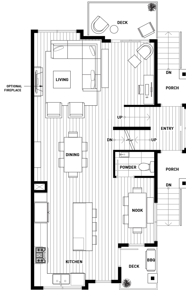
MAIN FLOOR
