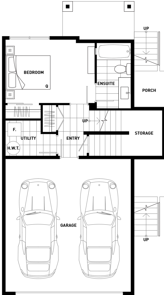
LOWER FLOOR
