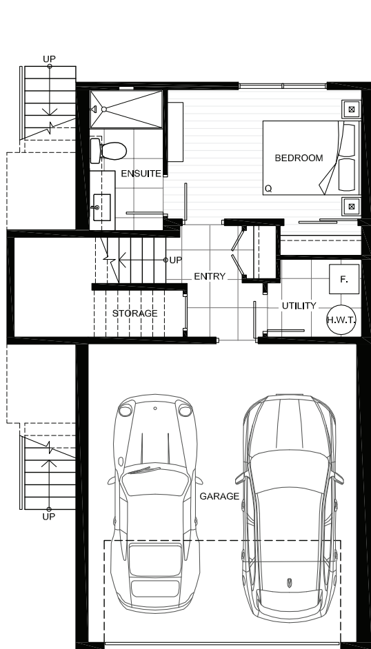
LOWER FLOOR
