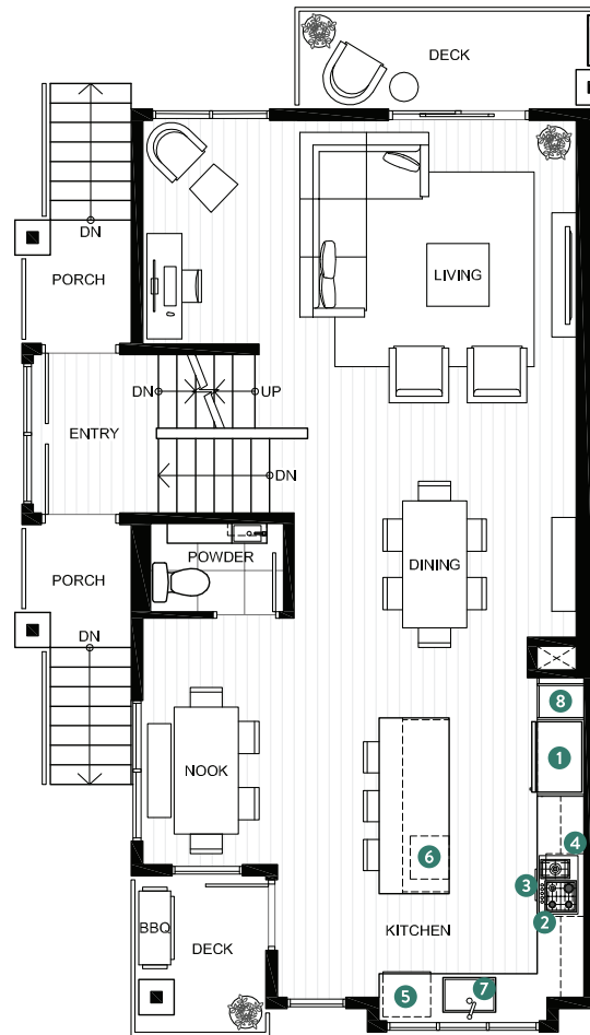
MAIN FLOOR
